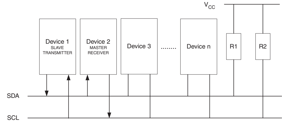
Figure 23-17. Data Transfer in Slave Transmitter Mode
