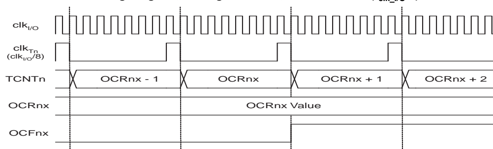
Figure 19-10. Timer/Counter Timing Diagram, Setting of OCF2A, with Prescaler ( f_{\text{clk}_{I/O}}/8 )
