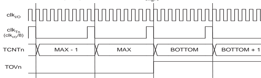
Figure 19-9. Timer/Counter Timing Diagram, with Prescaler ( f_{\text{clk}_{I/O}}/8 )
