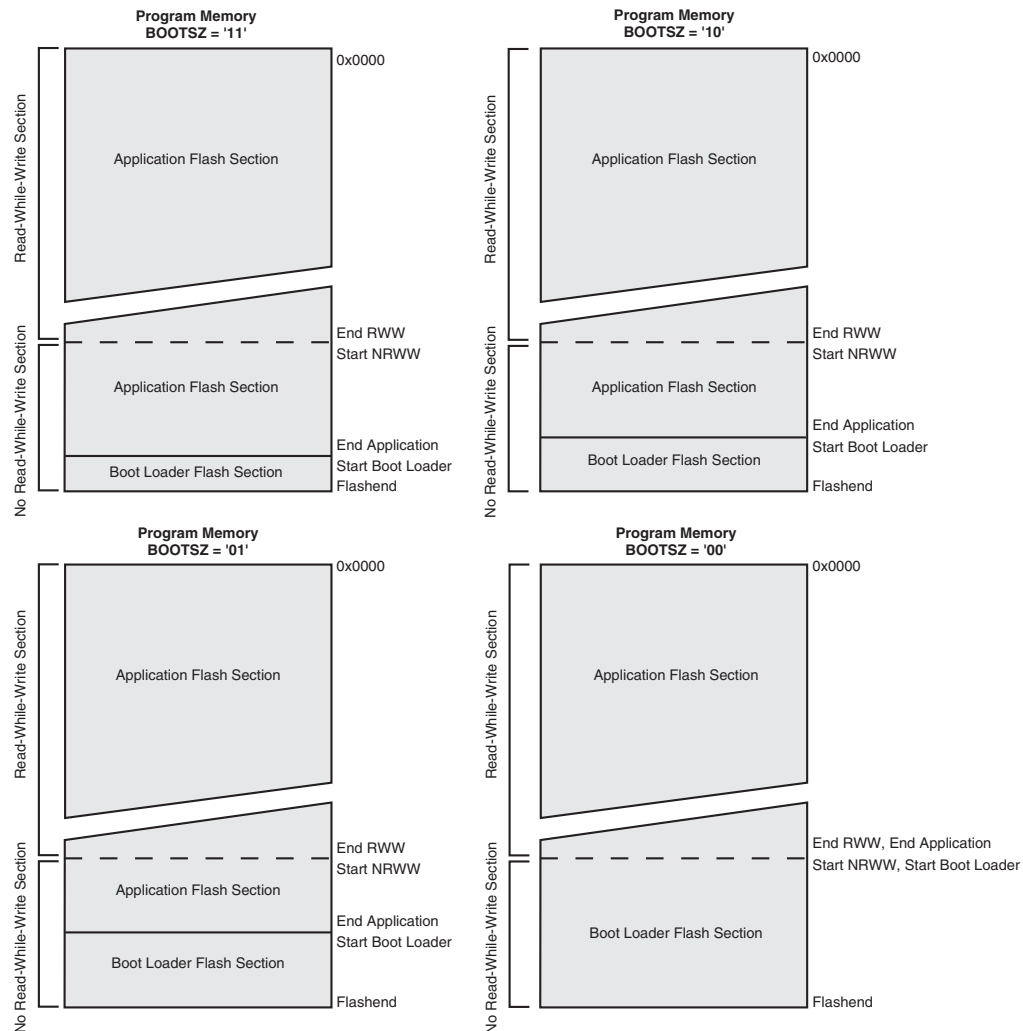
Figure 28-2. Memory Sections
