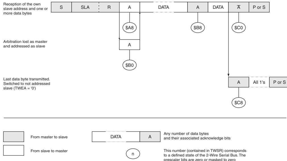
Figure 23-18. Formats and States in the Slave Transmitter Mode
