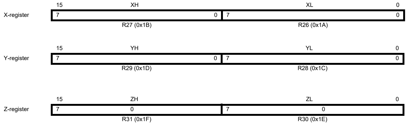
Figure 8-3. The X-, Y-, and Z-registers
