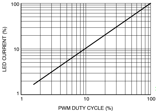
Figure 10. LED Current vs. PWM Duty Cycle
