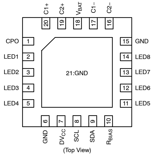
Figure 1. Pin Configuration
