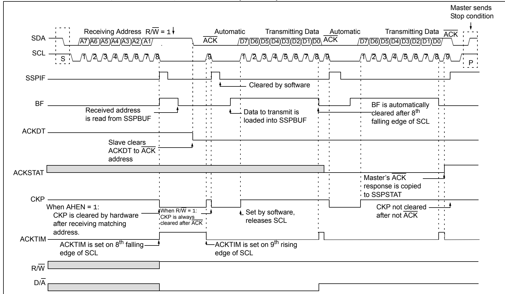
FIGURE 27-11: I 2 C SLAVE, 7-BIT ADDRESS, TRANSMISSION (AHEN = 1)
