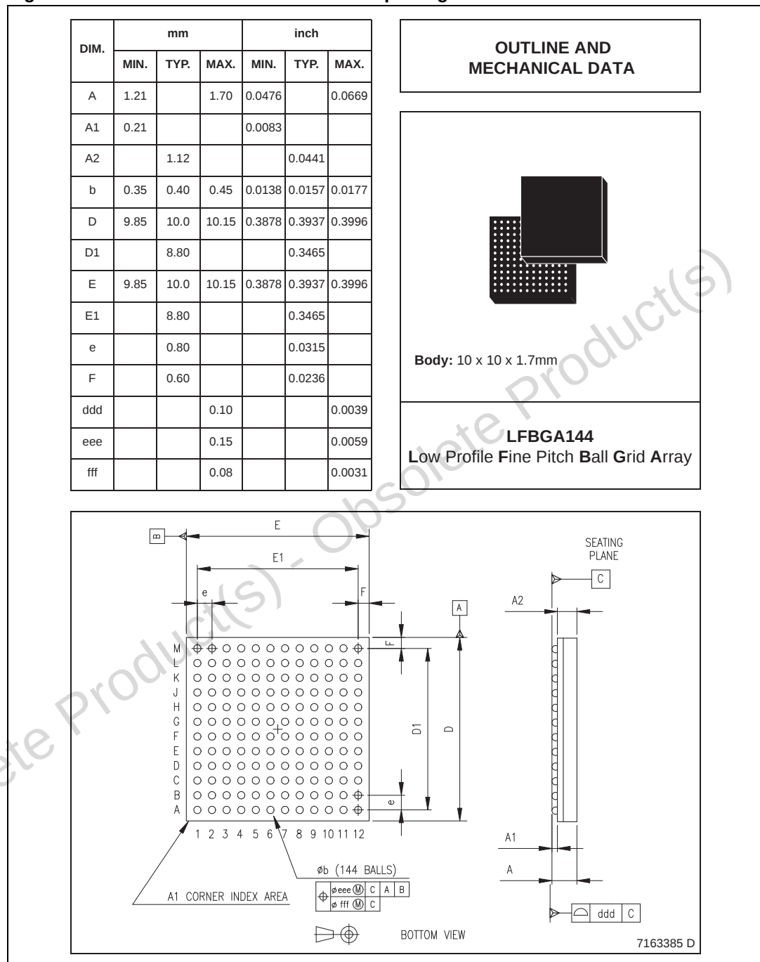
Figure 7. LFBGA144 mechanical data and package dimensions
