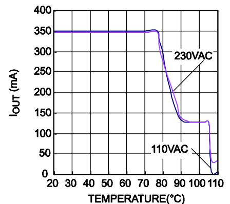
NTC Curve
