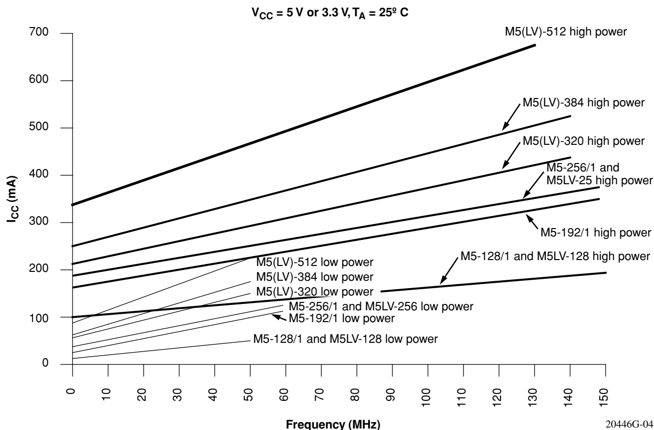
Figure 8. I_{CC} Curves at High/Low Power Modes
