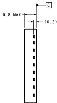
28-Pin Leadless Leadframe Package (LLP) NSC Package Number LQA28A
