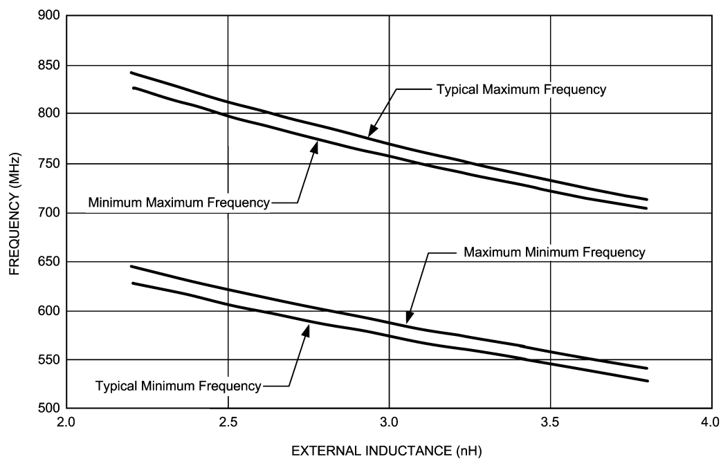
LMX2515LQ0701 Tuning Range vs. External Inductance (Note 12)
