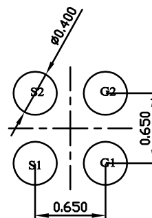
RECOMMENDED LAND PATTERN
