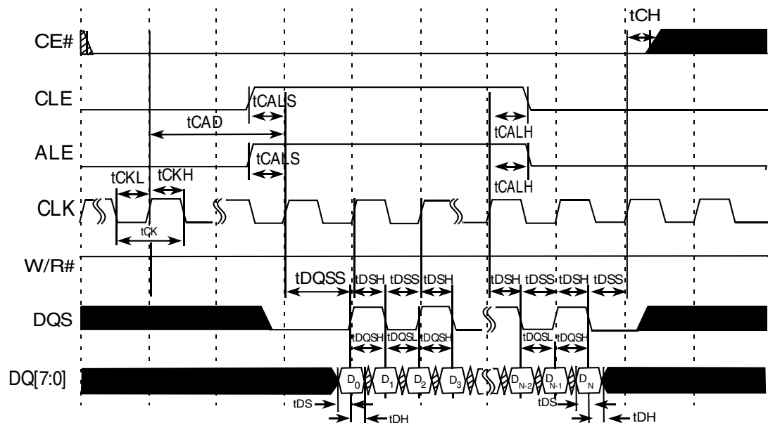
Figure 49. Write cycle
