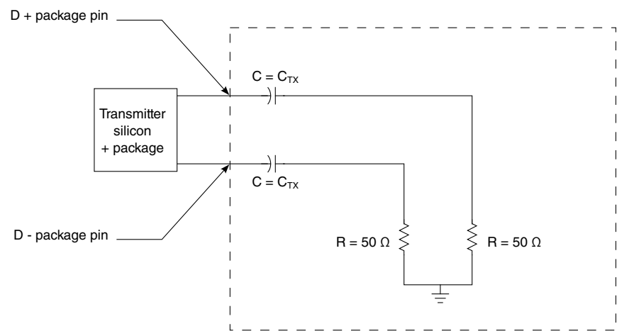
Figure 76. Test/measurement load
