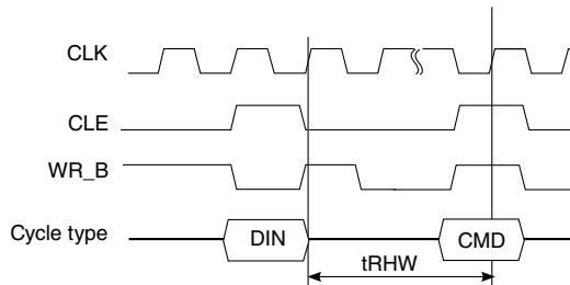
Figure 40. tRHW timings
