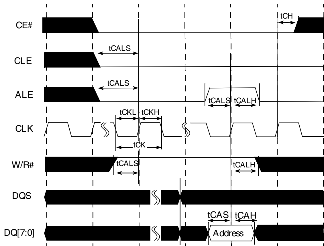
Figure 48. Address cycle
