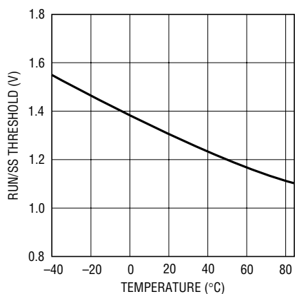
RUN/SS Threshold
