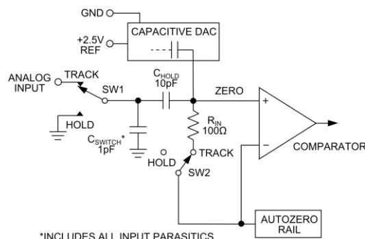
Figure 4: TSM1285 Equivalent Input Circuit Details.
