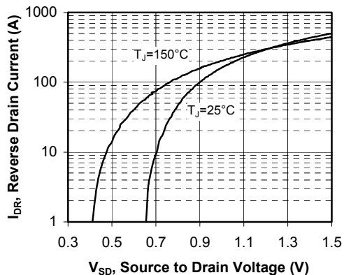
Source to Drain Diode Forward Voltage
