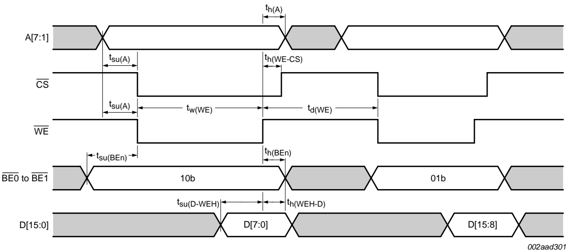
Fig 15. 8-bit write
