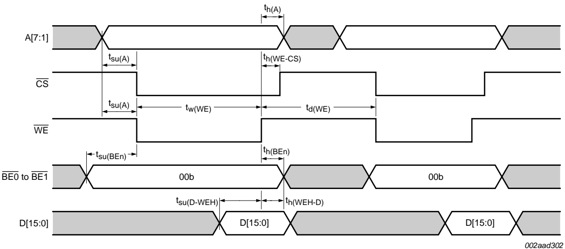
Fig 16. 16-bit write
