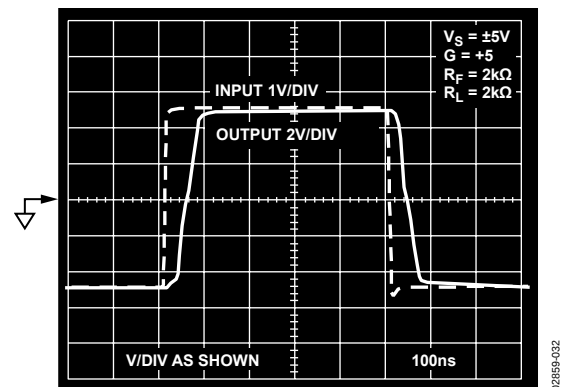
Figure 32. Overdrive Recovery
