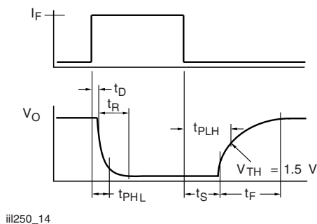
Fig. 14 - Switching Timing
