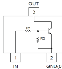
Device Schematic
