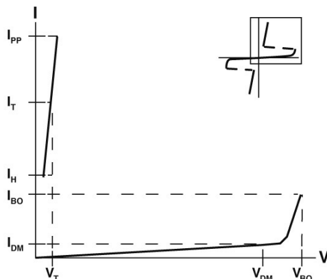
Figure SB1 - Voltage-Current Characteristics
