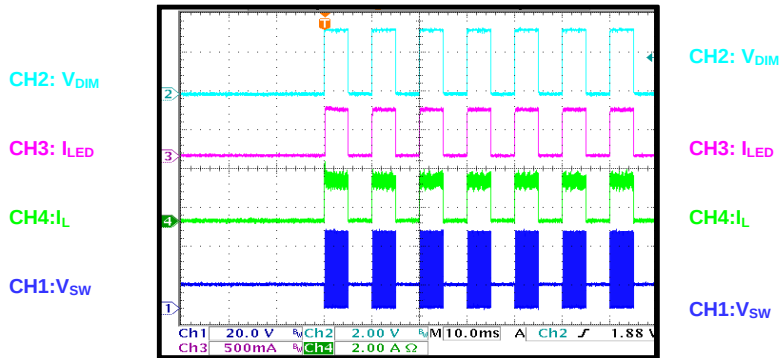
PWM Dimming On
