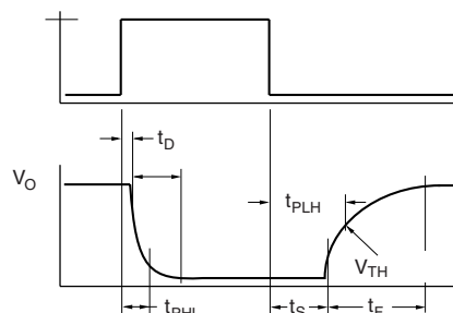
Fig. 3 - Saturated Switching Timing
