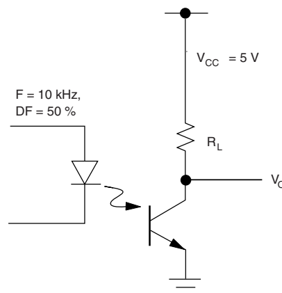
Fig. 4 - Saturated Switching Timing
