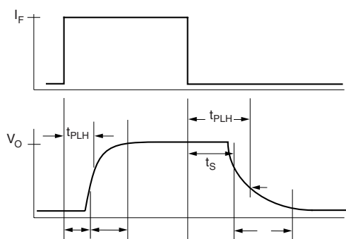
Fig. 1 - Non-Saturated Switching Timing
