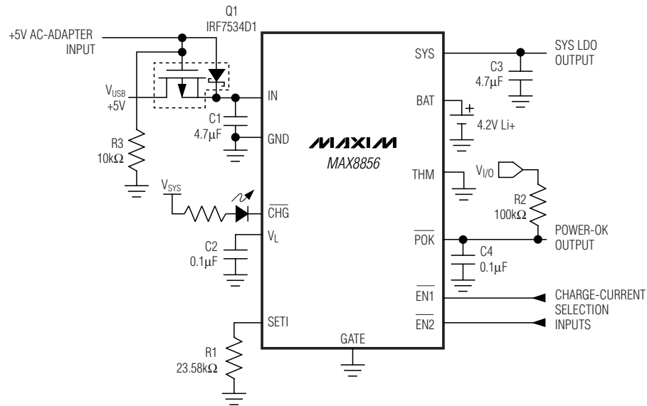
Figure 4. USB Application with AC Adapter
