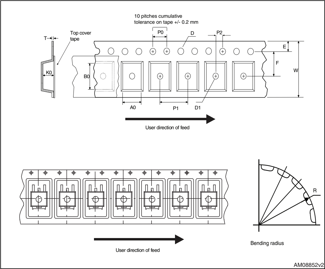
Figure 17. Tape dimension
