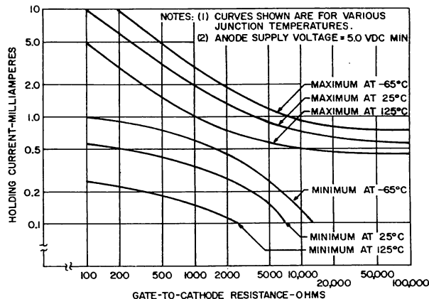
12. MAXIMUM AND MINIMUM HOLDING CURRENT VARIATION WITH EXTERNAL GATE-TO-CATHODE RESISTANCE FOR 2N2322-29 (C5 SERIES) ONLY
