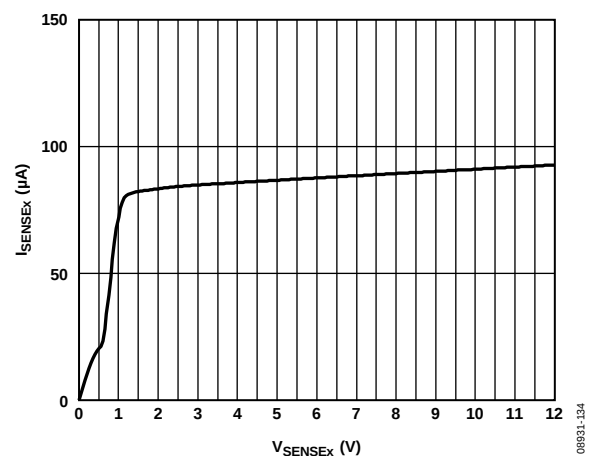
Figure 34. SENSE+ / SENSE- Input Current ( I_{SENSE} ) vs. Voltage ( V_{SENSE} )
