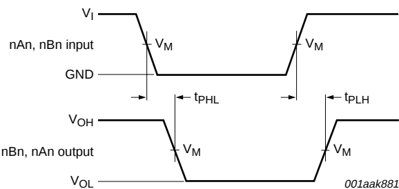
Measurement points are given in Table 8 . Logic levels: V_{OL} and V_{OH} are typical output voltage levels that occur with the output load.
