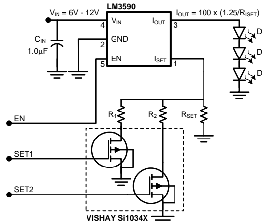
Figure 5. Example: R 1 = 15.8kΩ, R 2 = 31.6kΩ, R SET = 31.6kΩ
