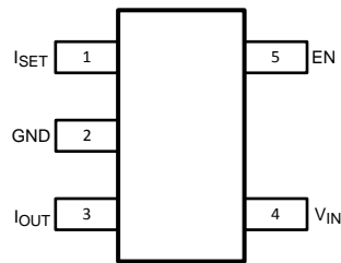
Figure 3. Top View
