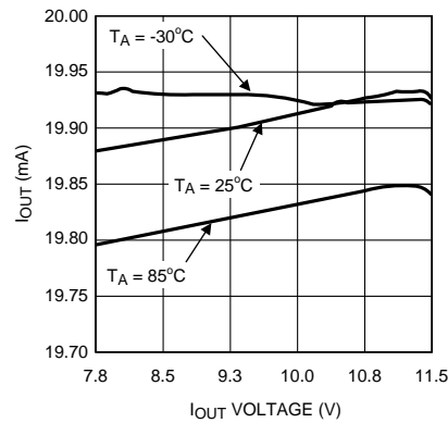
Figure 2. I OUT vs V OUT
