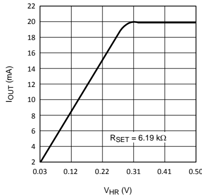
Figure 4. I OUT vs V HR V_{HR} = V_{IN} - V_{IOUT} V_{IN} = 12.0V
