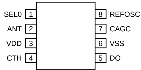
8-Pin SOP (M)
