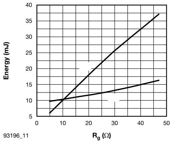
Fig. 11 - Typical IGBT Energy Loss vs. R_g T_J = 125^\circ\text{C} , I_C = 100\text{ A} , L = 500\text{ }\mu\text{H} , V_{CC} = 720\text{ V} , V_{GE} = 15\text{ V}
