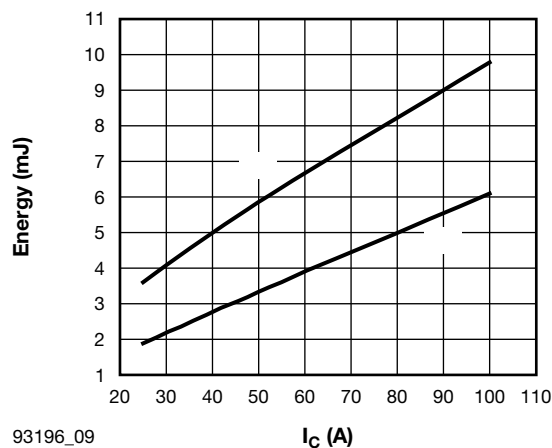
Fig. 9 - Typical IGBT Energy Loss vs. I_C T_J = 125\text{ }^{\circ}\text{C} , L = 500\text{ }\mu\text{H} , V_{CC} = 720\text{ V} , R_g = 5\text{ }\Omega , V_{GE} = 15\text{ V}
