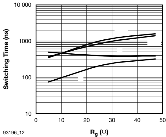
Fig. 12 - Typical IGBT Switching Time vs. R_g T_J = 125^\circ\text{C} , L = 500\text{ }\mu\text{H} , V_{CC} = 720\text{ V} , I_C = 100\text{ A} , V_{GE} = 15\text{ V}
