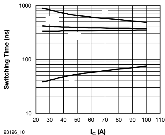
Fig. 10 - Typical IGBT Switching Time vs. I_C T_J = 125\text{ }^{\circ}\text{C} , L = 500\text{ }\mu\text{H} , V_{CC} = 720\text{ V} , R_g = 5\text{ }\Omega , V_{GE} = 15\text{ V}
