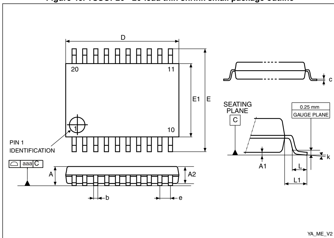
Figure 45. TSSOP20 - 20-lead thin shrink small package outline
