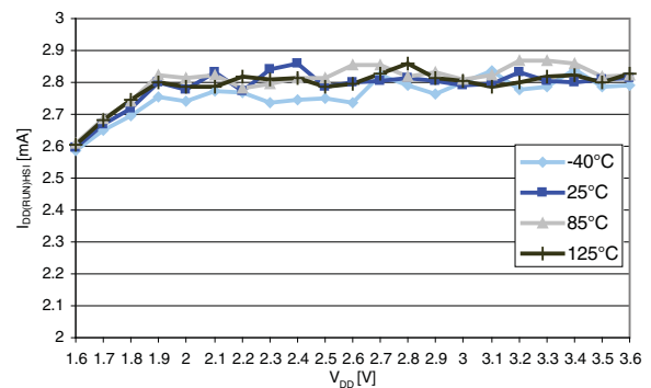
Figure 12. I_{DD(RUN)} vs. V_{DD} , f_{CPU} = 16\text{ MHz}
