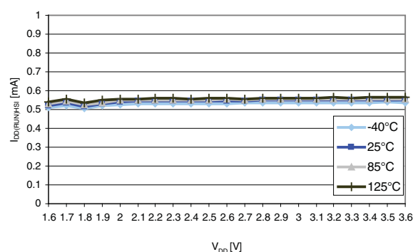
Figure 11. I_{DD(RUN)} vs. V_{DD} , f_{CPU} = 2\text{ MHz}
