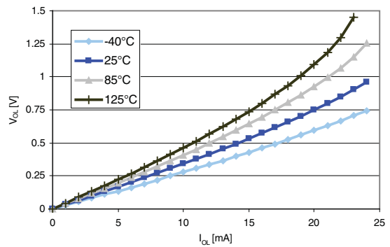
Figure 24. Typ. V_{OL} at V_{DD} = 3.0 V (High sink ports)
