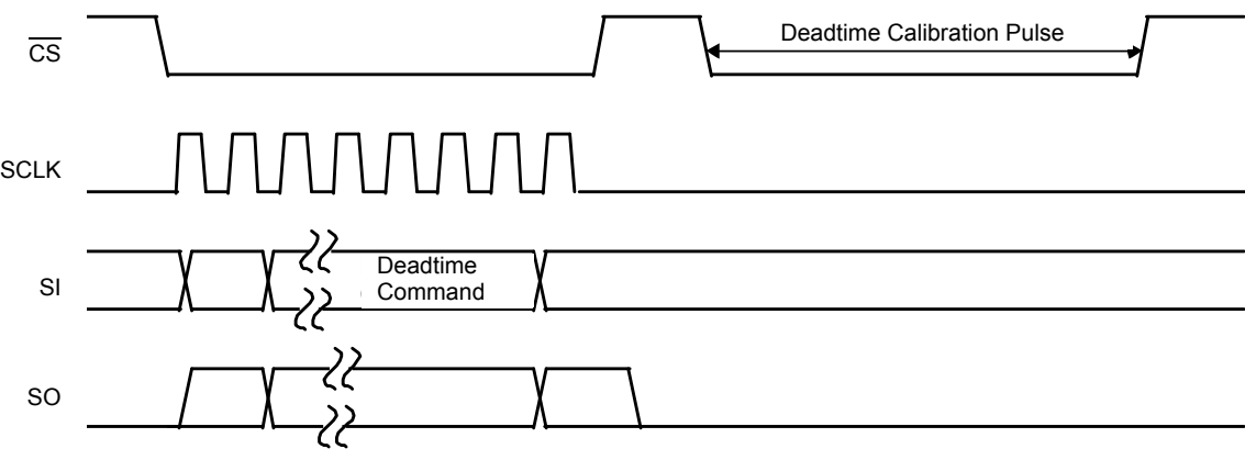
Figure 19. Deadtime calibration
