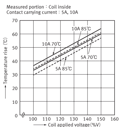
3-2. Coil temperature characteristics (1 Form C)
