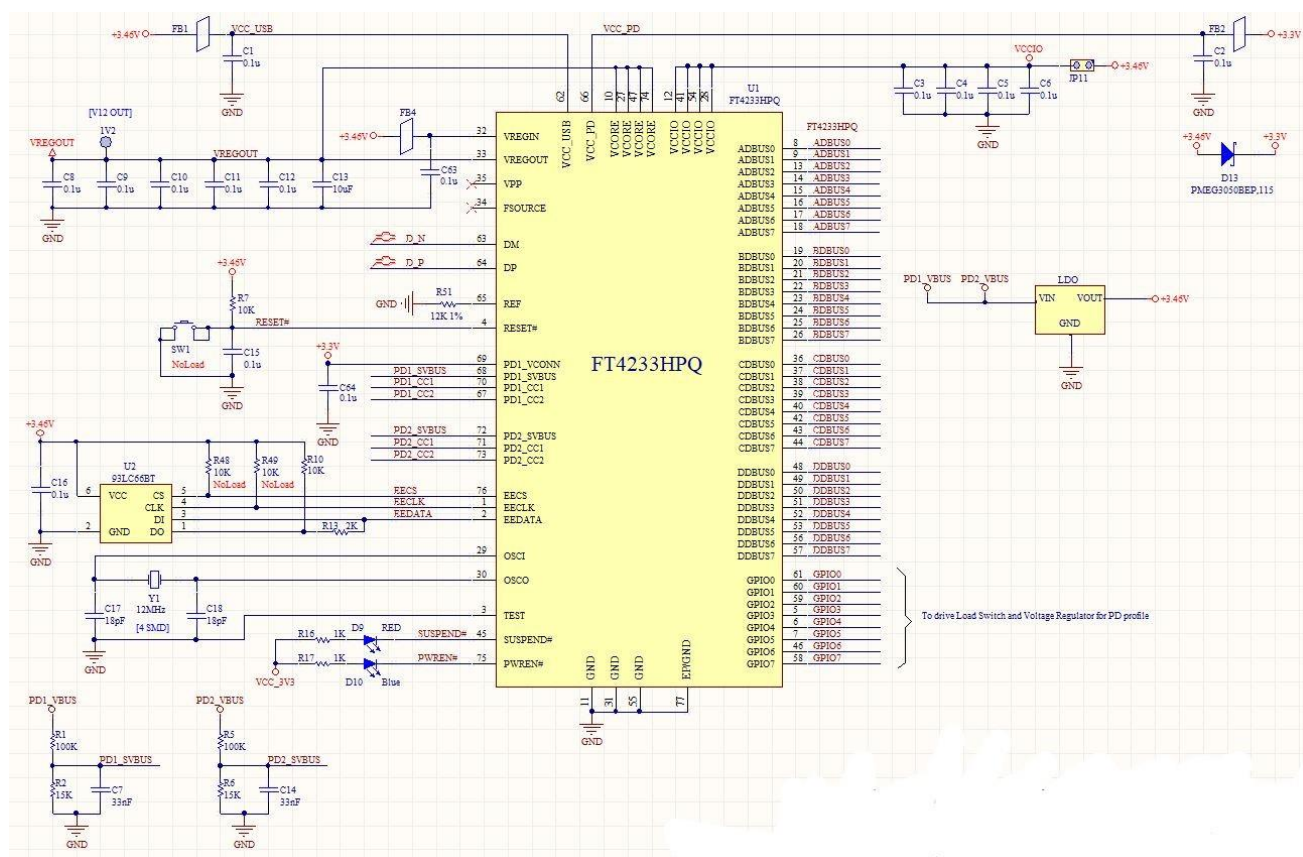
Figure 19 - Bus Power PD Configuration Diagram
