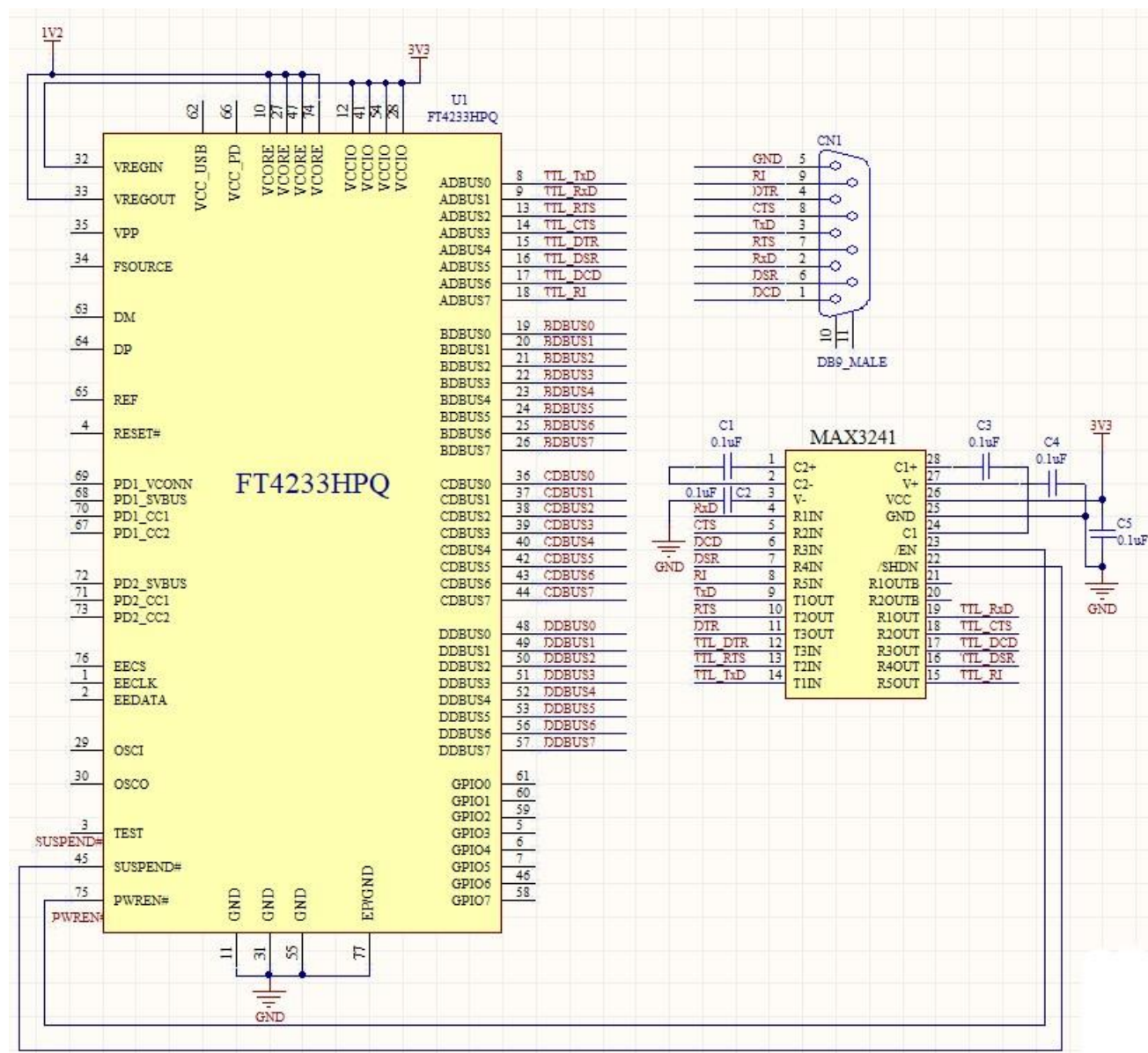
Figure 5 - Single RS232 Configurations
