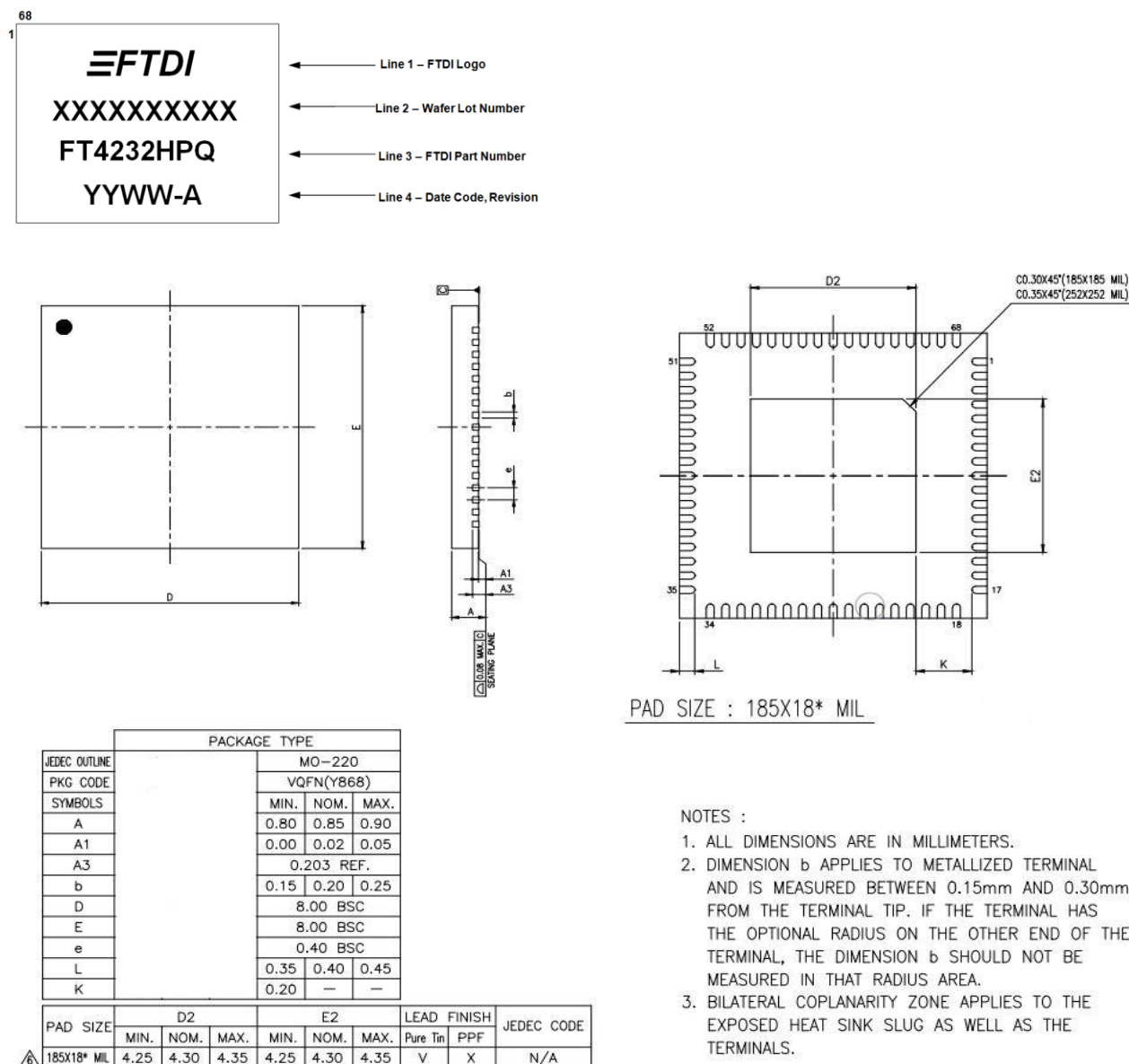
Figure 16 - 68 Pin QFN Package Details
