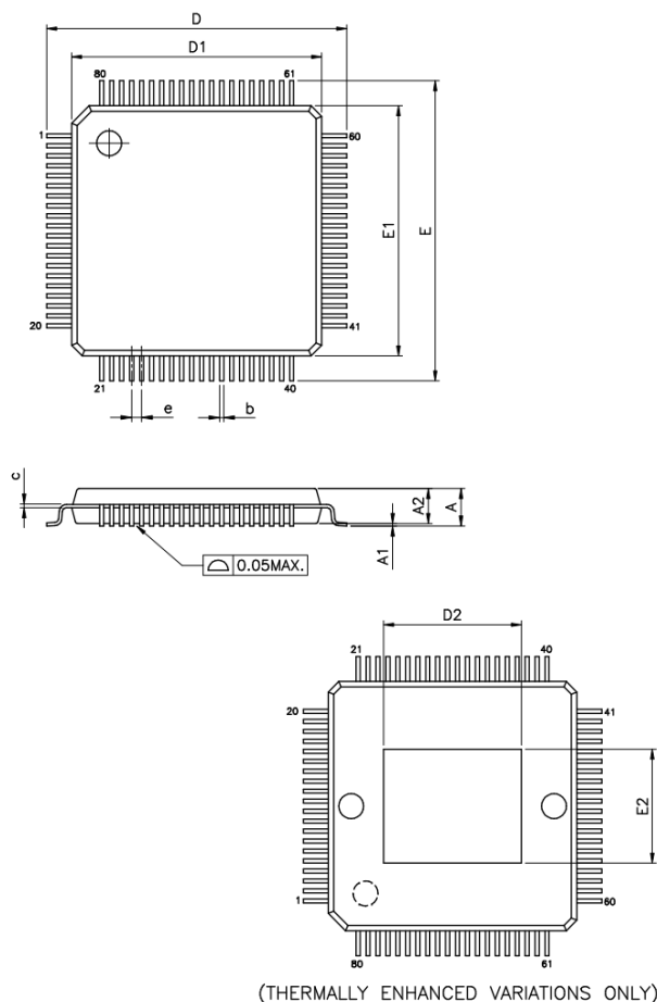
Figure 14 - 80 Pin LQFP Package Details
