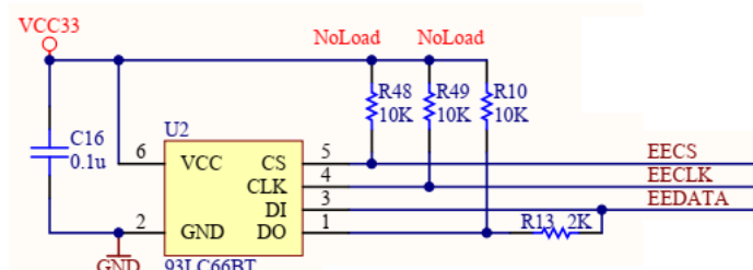
Figure 20 - EEPROM Interface
