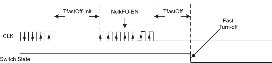
Figure 3: High-speed Turn-off Mode
