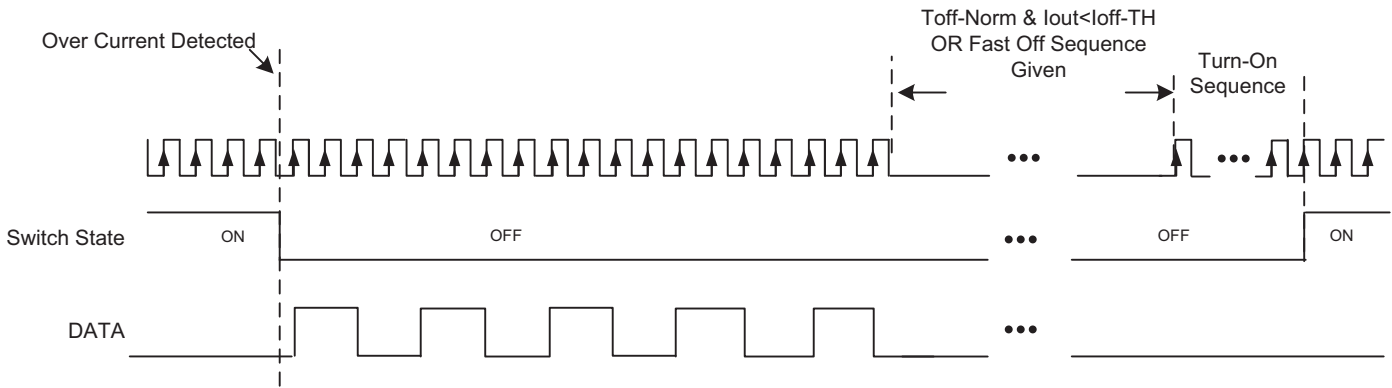
Figure 4: Over-current Shut-down and Restart
