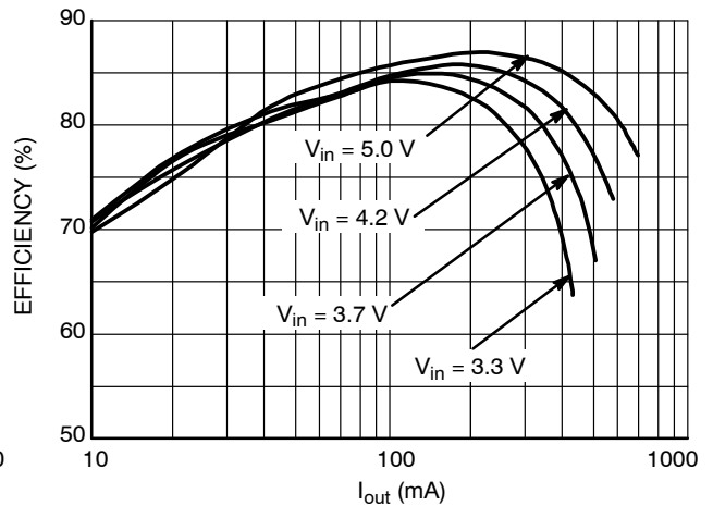
Figure 7. Efficiency vs. Current @ 3 LEDs (10.5 V @ 350 mA), L = \text{TDK VLF5014A-2R7M1R5} , (Notes 13 and 14)
