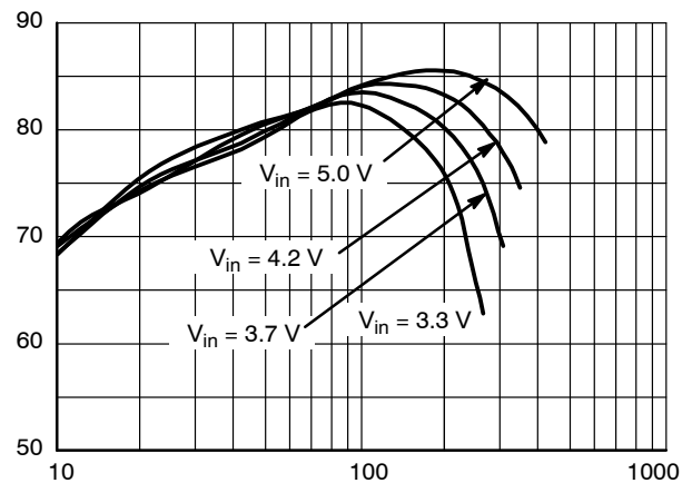
Figure 9. Efficiency vs. Current @ 5 LEDs (17.5 V @ 350 mA), L = \text{TDK VLF5014A-2R7M1R5} (Notes 13 and 14)
