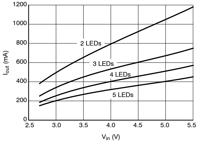
Figure 5. Typical Maximum Output Current vs. Input Voltage, L = \text{TDK VLF5014A-2R7M1R5} (Note 13)
