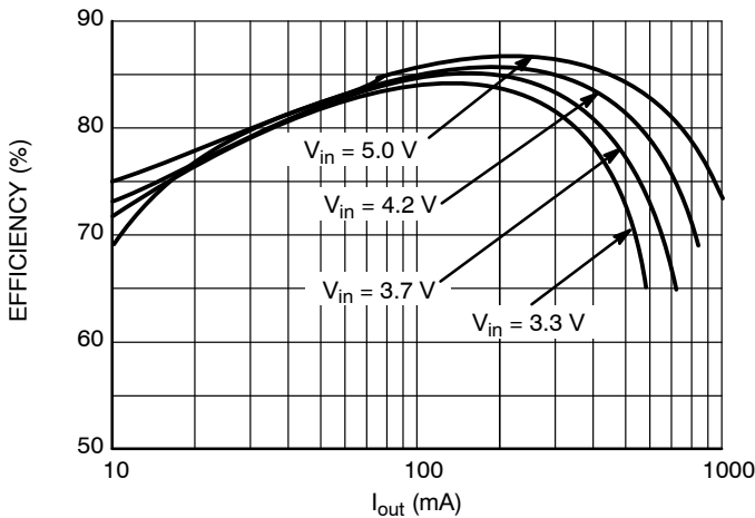
Figure 6. Efficiency vs. Current @ 2 LEDs (7.0 V @ 350 mA), L = \text{TDK VLF5014A-2R7M1R5} , (Notes 13 and 14)
