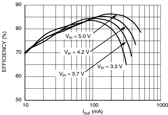
Figure 8. Efficiency vs. Current @ 4 LEDs (14 V @ 350 mA), L = \text{TDK VLF5014A-2R7M1R5} , (Notes 13 and 14)
