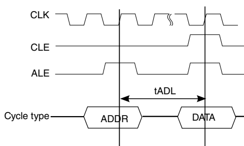
Figure 51. tADL timings
