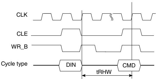
Figure 53. t_{RHW} timings
