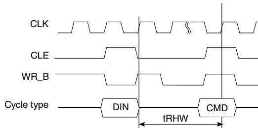
Figure 40. t_{RHW} timings
