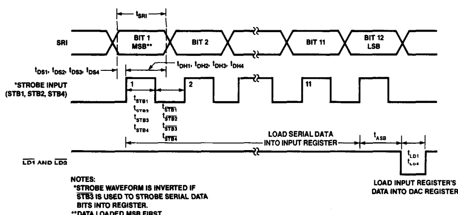
FIGURE 6: Timing Diagram
