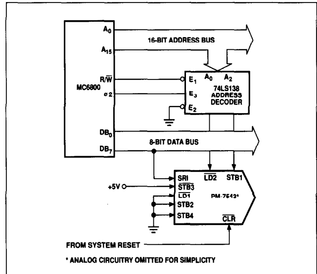
FIGURE 11: PM-7543 - MC6800 Interface
