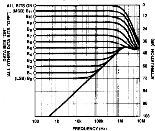
MULTIPLYING MODE FREQUENCY RESPONSE vs DIGITAL CODE
