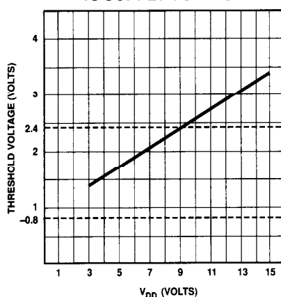
LOGIC THRESHOLD VOLTAGE vs SUPPLY VOLTAGE
