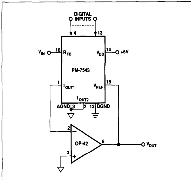
FIGURE 10: Analog/Digital Divider
