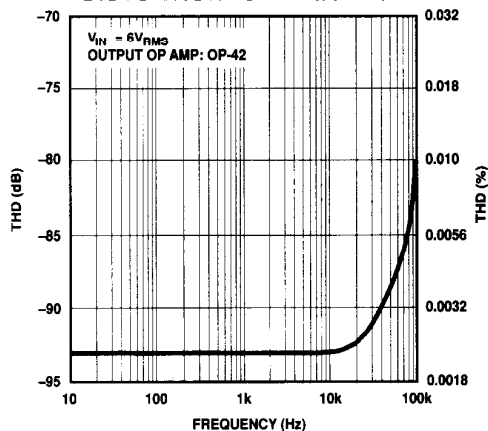
MULTIPLYING MODE TOTAL HARMONIC DISTORTION vs FREQUENCY
