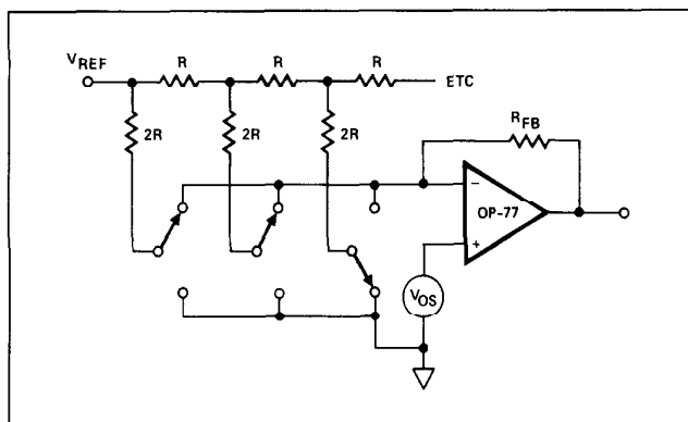
FIGURE 5: Simplified Circuit
