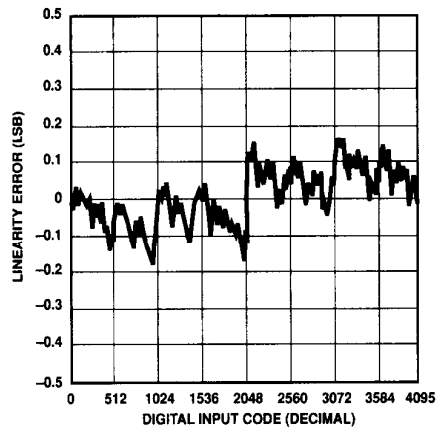
LINEARITY ERROR vs DIGITAL CODE
