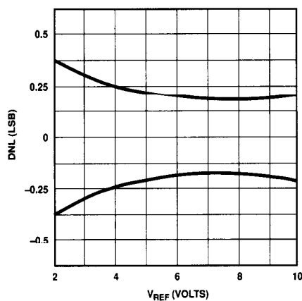
DNL ERROR vs REFERENCE VOLTAGE
