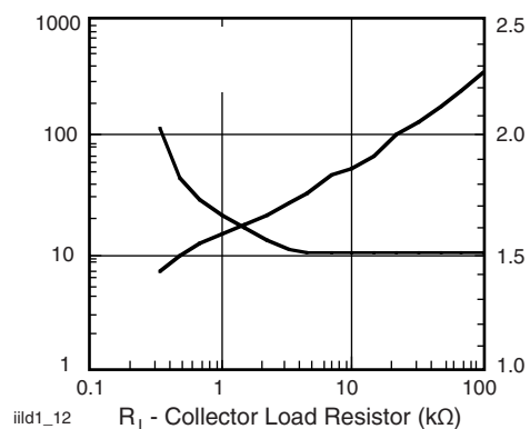
Fig. 14 - Propagation Delay vs. Collector Load Resistor
