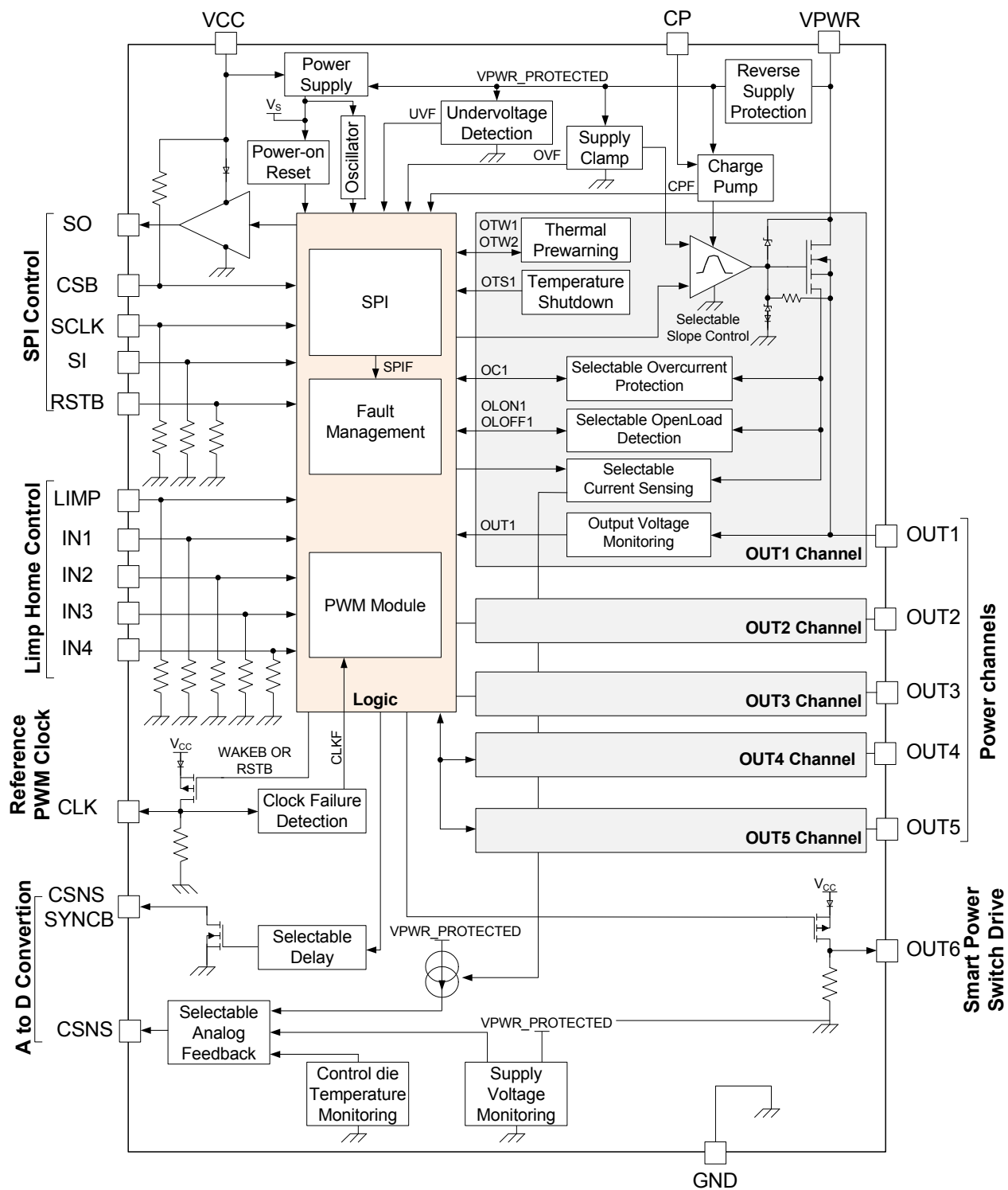
Figure 2. 12XSFD simplified internal block diagram (penta version)
