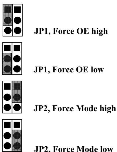
Figure 2. JP1-JP2 Jumper Positions
