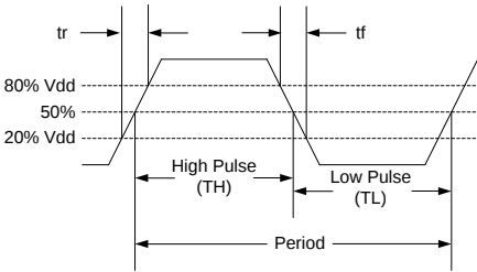
Figure 3. Output Waveform
