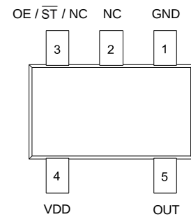
Figure 1. Pin Assignments
