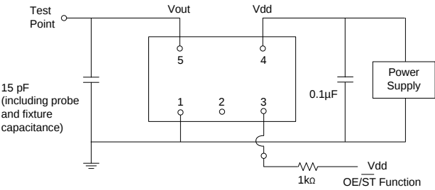
Figure 2. Test Circuit
