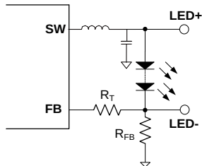
Figure 4: Feedback Network
