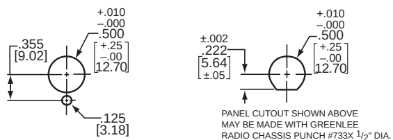
Mounting Details with Locking Ring
