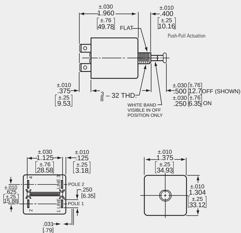
Push-Pull, Two Pole
