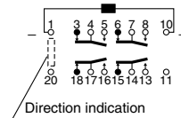
1-coil latching
