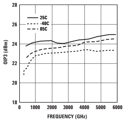
Figure 14. OIP3 vs. Frequency (3V 20 mA).
