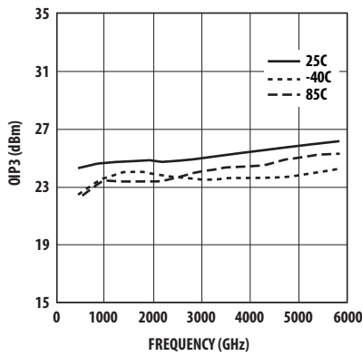
Figure 22. OIP3 vs. Frequency (5V 20 mA).
