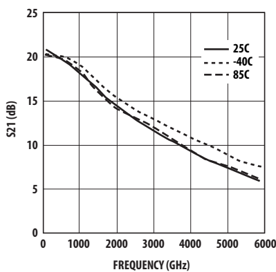
Figure 20. S21 vs. Frequency (5V 20 mA).
