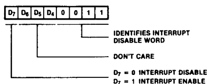
Figure 11. Interrupt Disable Word
