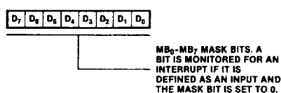
Figure 10. Mask Control Word
