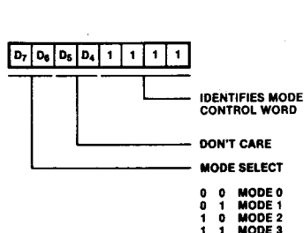
Figure 6. Mode Control Word
