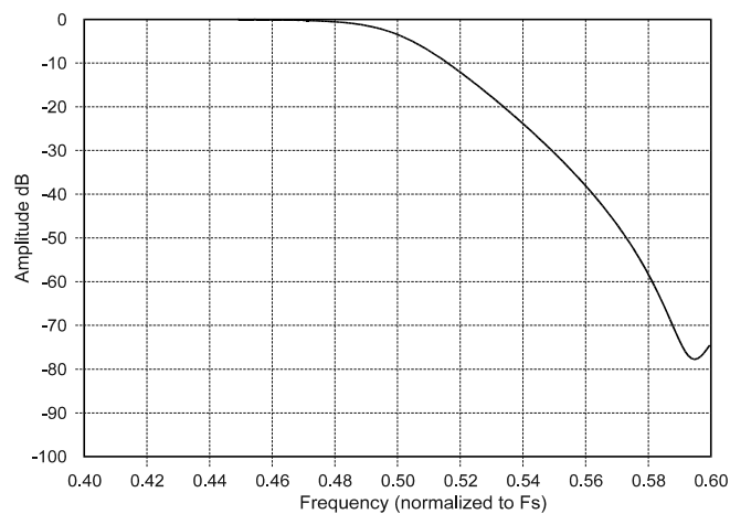
Figure 20. Transition Band
