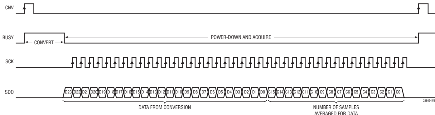
Figure 22. Serial Output Code Parsing
