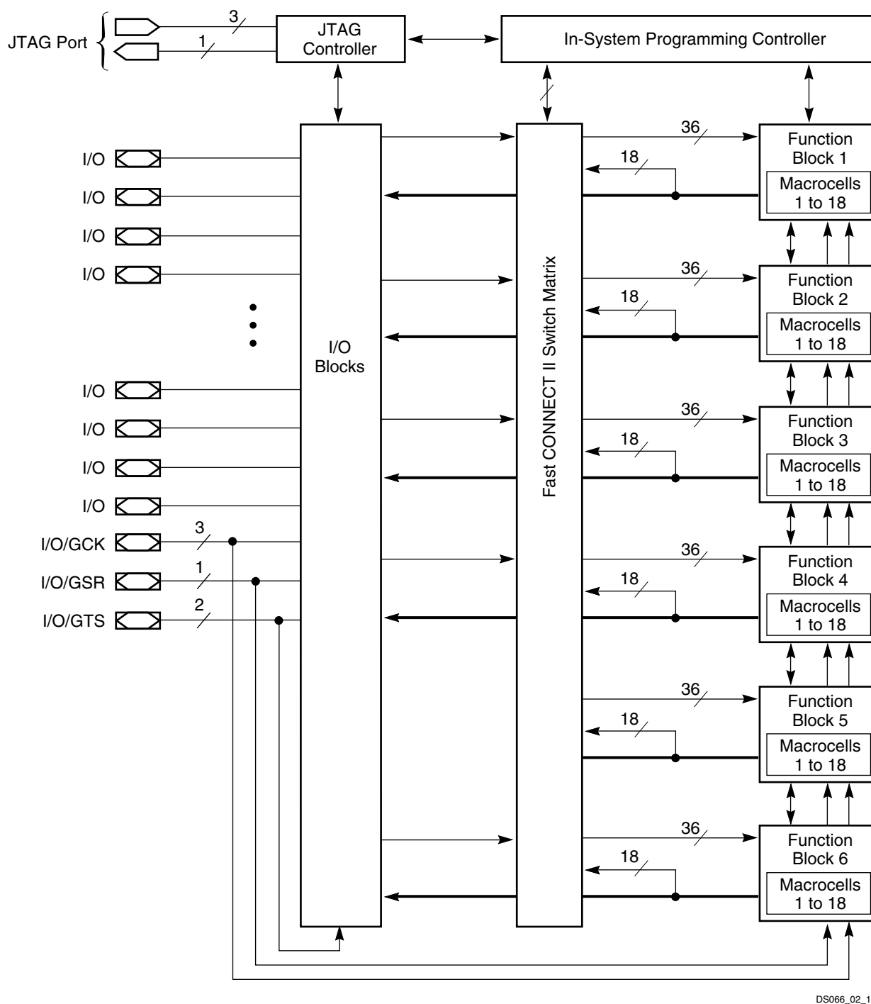
Figure 2: XC95108 Architecture
