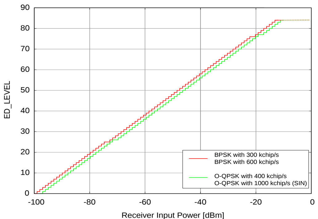
Figure 8-22. Mapping between ED Value and Receiver Input Power.
