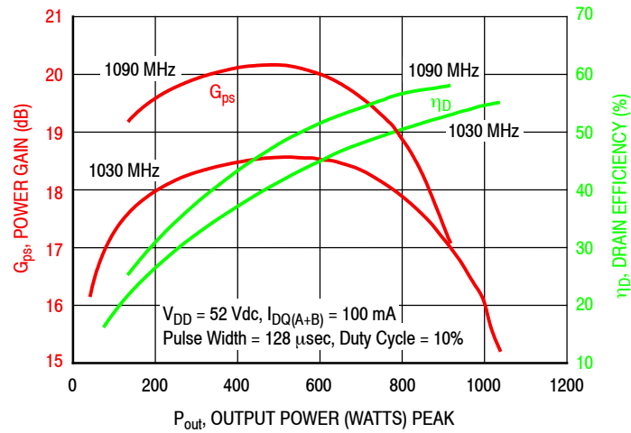
Figure 7. Power Gain and Drain Efficiency versus Output Power – 52 V
