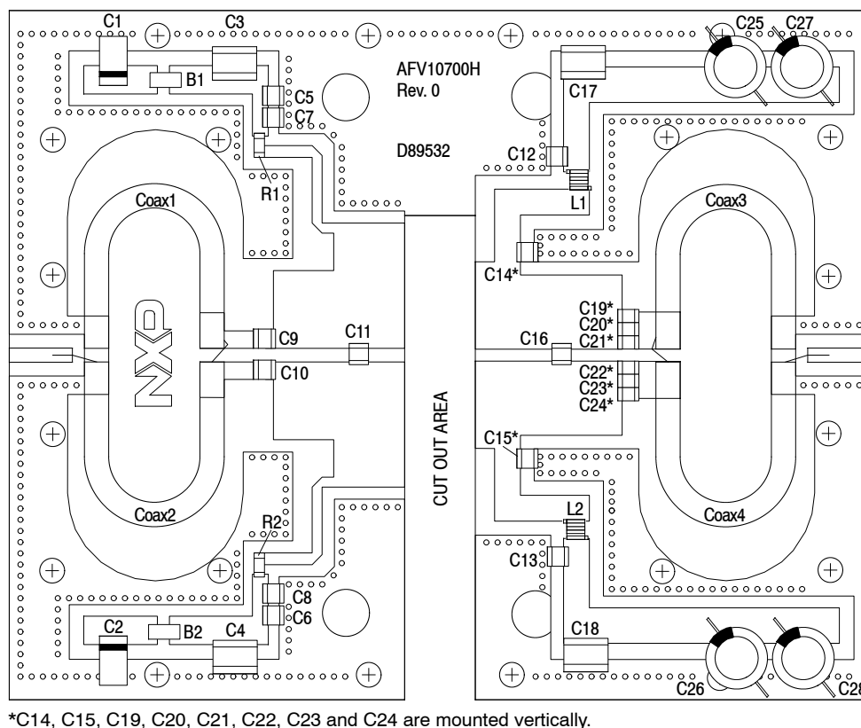
Figure 9. AFV10700H Narrowband Test Circuit Component Layout – 1030 MHz
