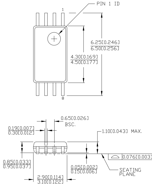
Figure 6. 8-pin TSSOP (4.40 mm Body) Z08.173/ZZ08.173, 51-85093
